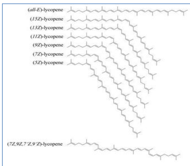
Figure 1: (all- E -) Isomer and some ( Z -) isomers of lycopene.
