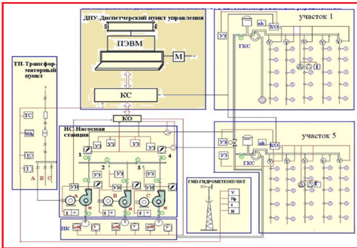
Figure 1: Schematic diagram of a pulse sprinkler system of self-oscillating action with automated control
